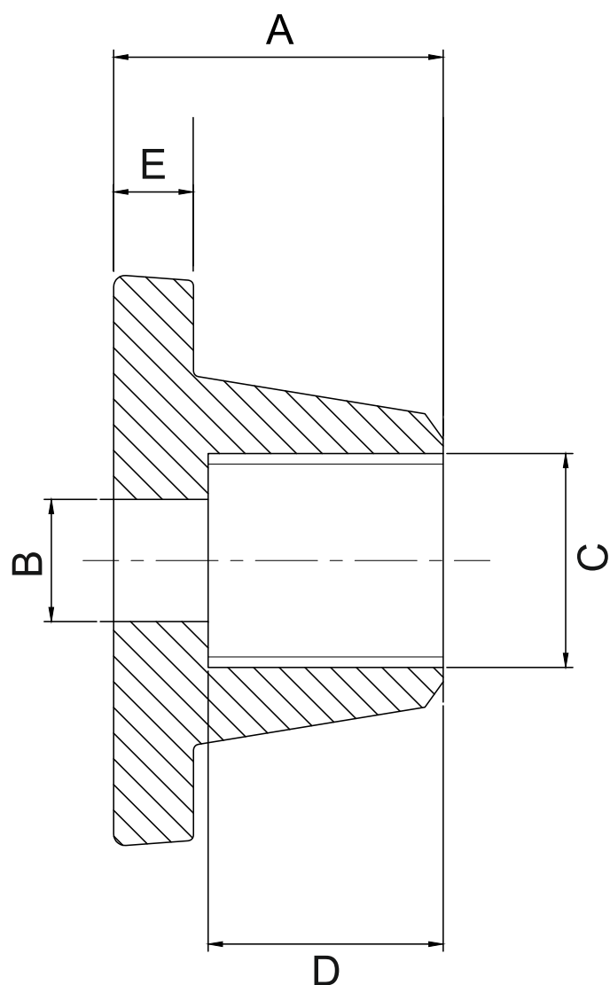
DIMENSIONAL DETAILS OF 3 PIECE (RB) SCREWED/SOCKET-WELD END PIECE
